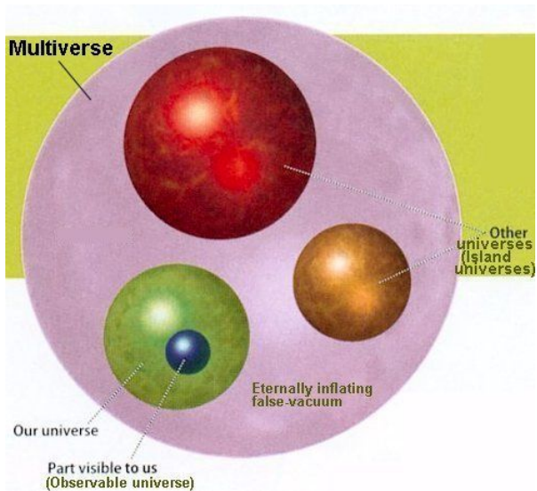
Multiverse -4
