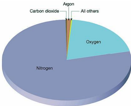
Principal gases of dry air
