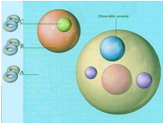
Multiverse -2
