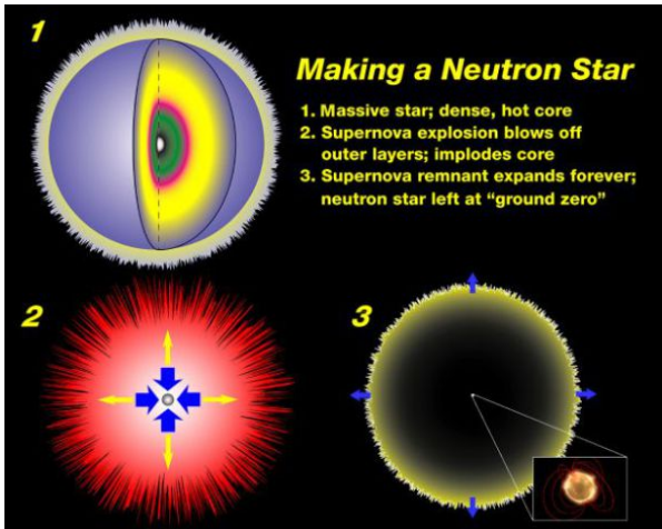
Making a neutron star
