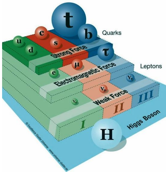
Particles Forces
