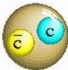
J/\psi
