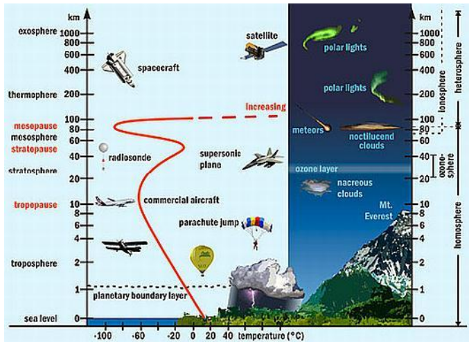
Vertical structure of the Earth's Atmosphere
