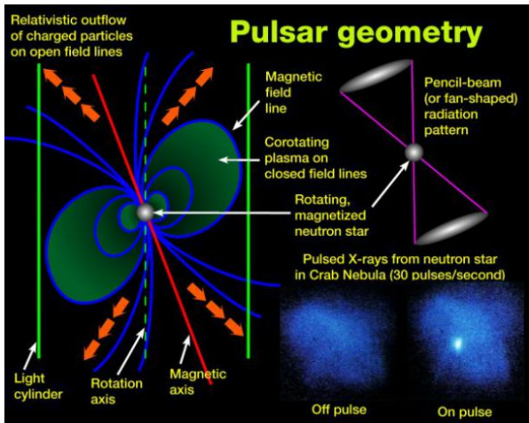
Pulsar geometry
