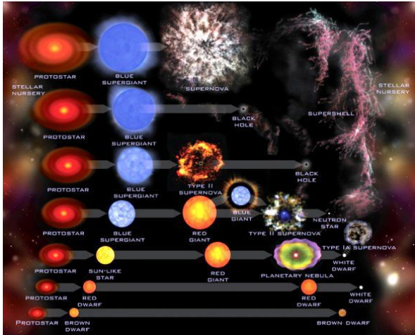
Stellar Evolution
