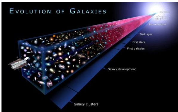
Galaxies -6
